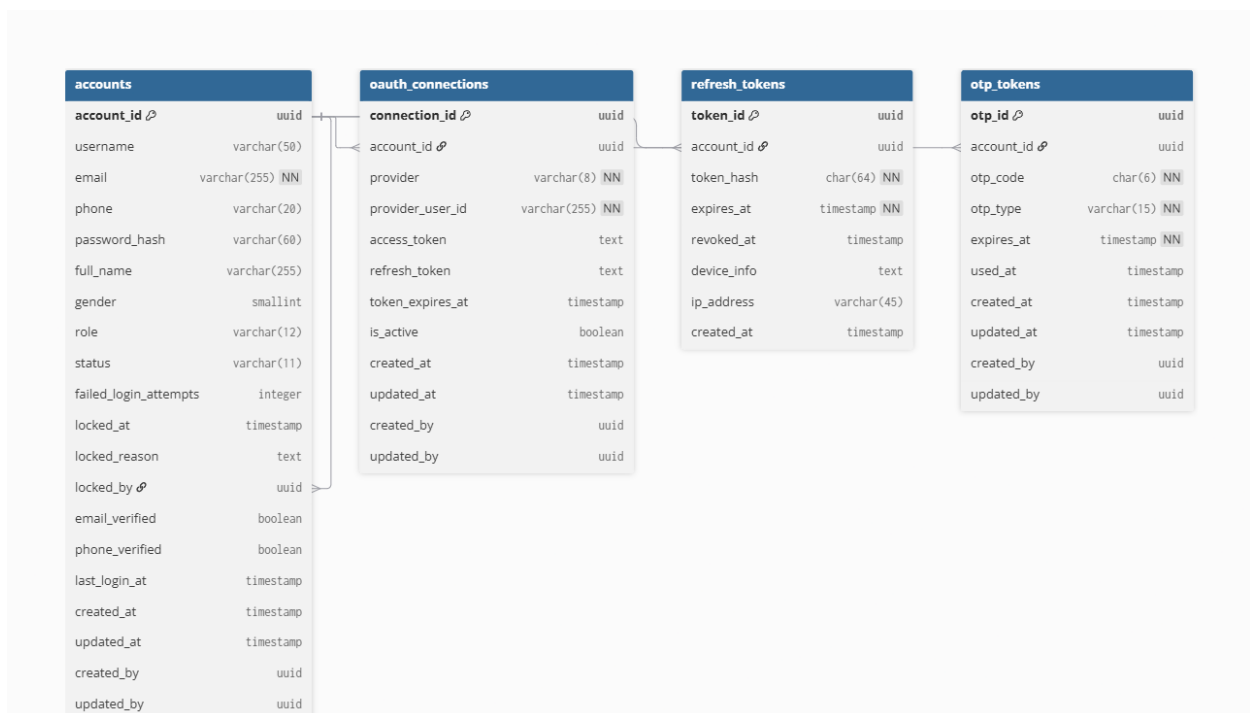
Figure 1. Auth Service Database
